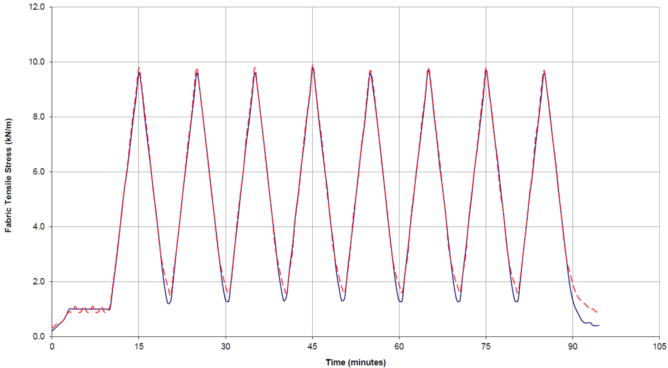
Load Diagram
