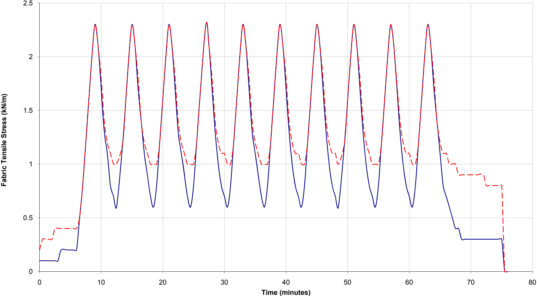
Load Diagram
