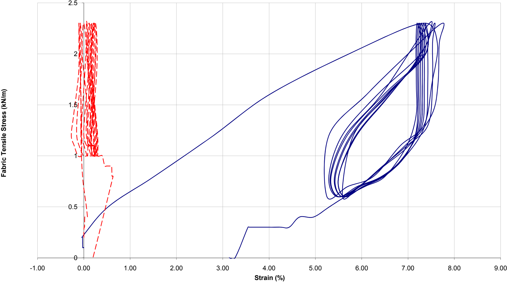
Biaxial Elongation — Warp - - - Fill
