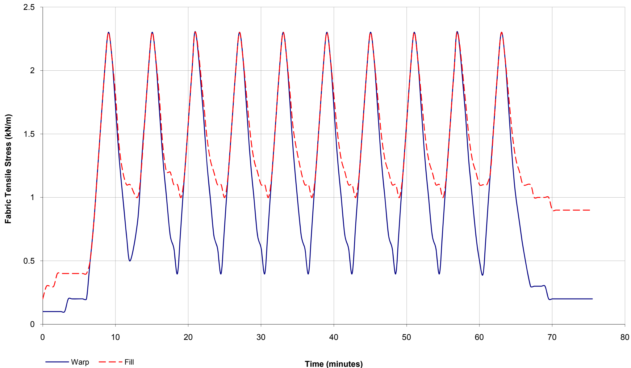
Load Diagram
